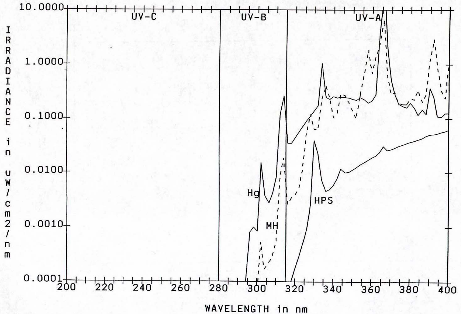
FIGURE 14 UV SPECTRAL IRRADIANCE AT 1000 LUX FOR 400 W HG, MH AND HPS LAMPS
